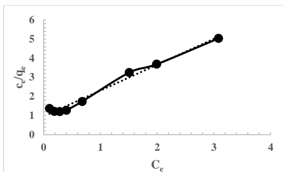
Fig 8. Langmuir isotherm plot for adsorption of RhB onto 3A zeolite
