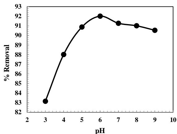
Fig 4. Effect of pH of sample solution on adsorption of RhB onto 3A zeolite
