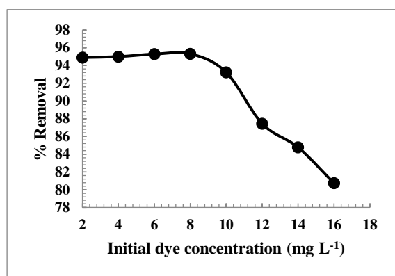
Fig 6. Effect of initial dye concentration on adsorption of RhB onto 3A zeolite
