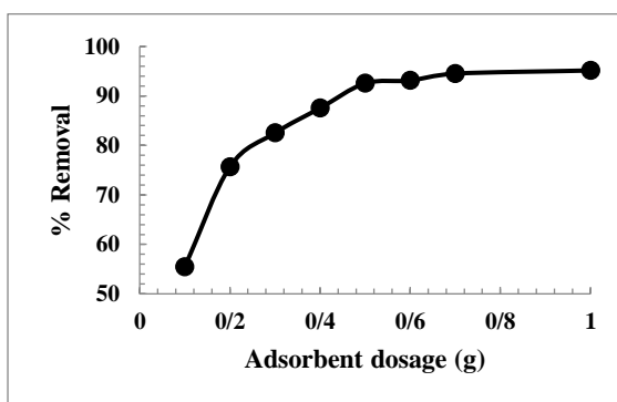
Fig 5. Effect of adsorbent dosage on adsorption of RhB onto 3A zeolite
