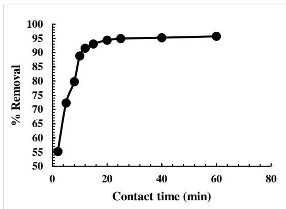
Fig 7. Effect of contact time on adsorption of RhB onto 3A zeolite
