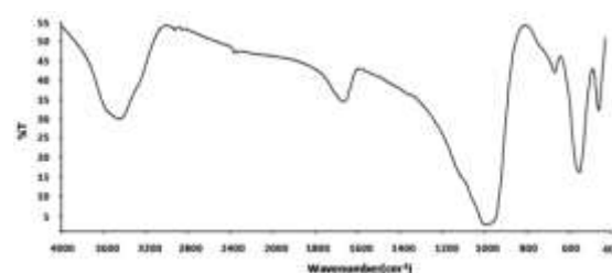
Fig 2. FTIR spectra of 3A zeolite
