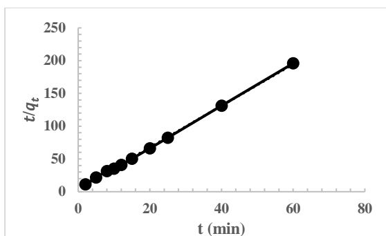
Fig 9. Pseudo second-order kinetic plot for adsorption of RhB onto 3A zeolite
