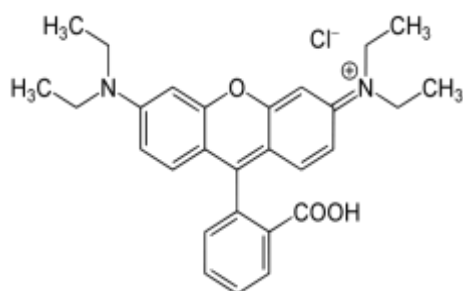
Fig 1. Chemical structure of RhB
