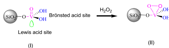
Figure 1. Silica Vanadic Acid (SVA) (I) in situ converted to peroxovanadium species (II) in the presence of H 2 O 2 (II)
