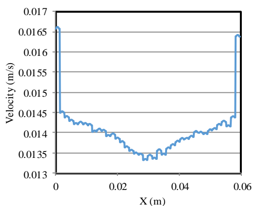
Fig 7. Velocity distribution counter (a) and velocity diagram (b) in “A” type micro-channel reactor
