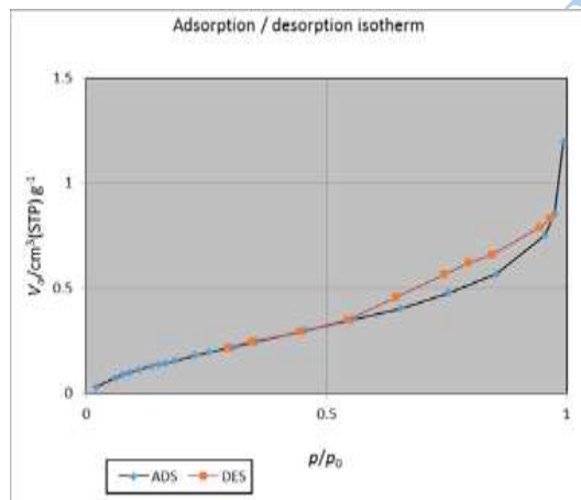
Fig 5. \text{N}_2 adsorption-desorption isotherm plot
