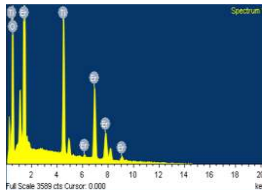
Fig 3. EDX analysis of the \text{Er}_2\text{Ti}_2\text{O}_7 sample.
