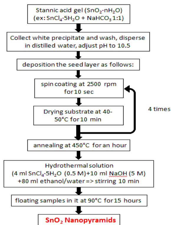
Scheme 1. All preparation steps of SnO 2 nanopyramids
