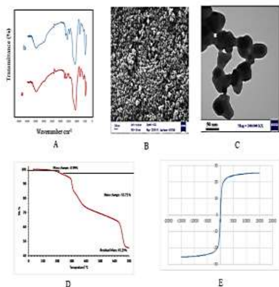
Figure 1. FT-IR spectra of Fe 3 O 4 and Fe 3 O 4 @SiO 2 @PAMAM-G2 (A), FE-SEM images of Fe 3 O 4 @SiO 2 @PAMAM-G2 (B), TEM images of Fe 3 O 4 @SiO 2 @PAMAM-G2 (C), TGA of Fe 3 O 4 @SiO 2 @PAMAM-G2 (D), VSM of Fe 3 O 4 @SiO 2 @PAMAM-G2 (E).
