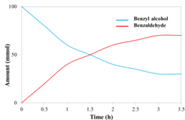
Fig. 12. Experimental results of oxidation of benzyl alcohol by henna sensitized n-TiO 2 -P25 under blue light irradiation.
