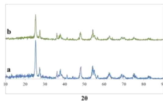
Fig. 3. XRD patterns of a) n-TiO 2 -P25, and b) Henna sensitized n-TiO 2 -P25.
