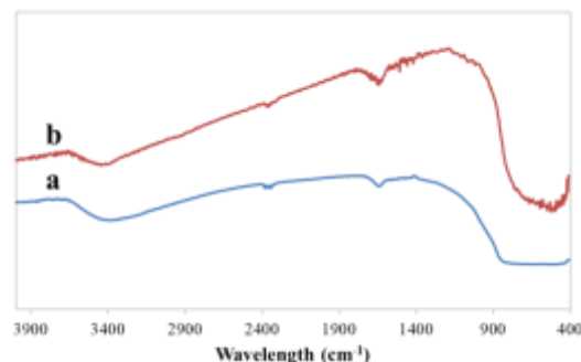
Fig. 2. The FT-IR spectra of a) bare n-TiO 2 -P25 and b) henna sensitized n-TiO 2 -P25.
