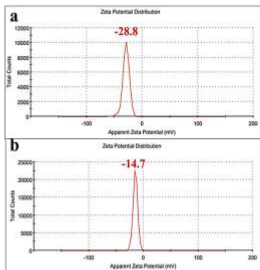
Fig. 9. Zeta potential determination of a) bare n-TiO 2 -P25 and b) henna sensitized n-TiO 2 -P25.
