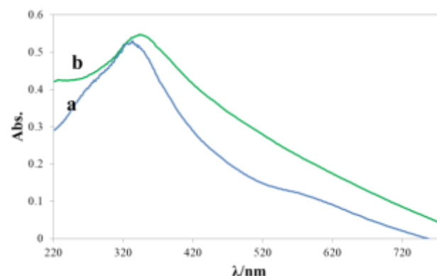
Fig. 10. UV-Visible absorption spectra of a) bare n-TiO 2 -P25 and b) henna sensitized n-TiO 2 -P25.
