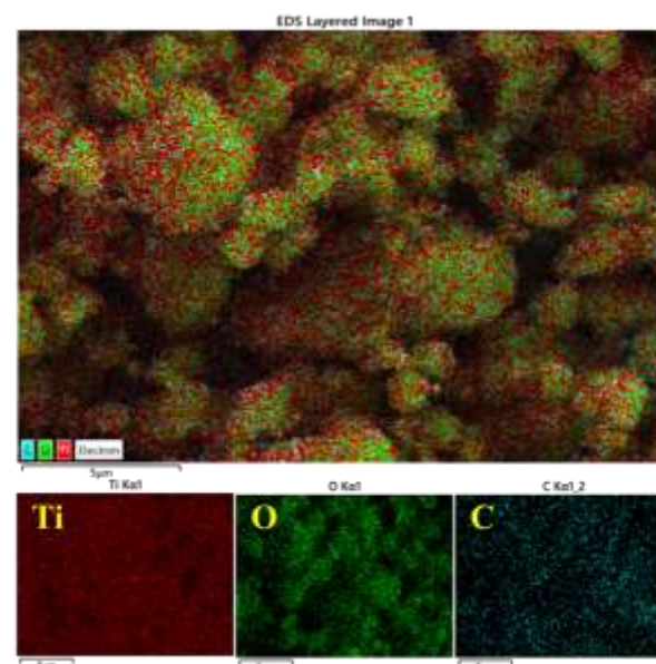
Fig. 6. Elemental mapping analysis of henna sensitized n- \text{TiO}_2 -P25.
