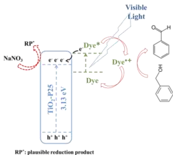
Fig. 13. Possible mechanism of oxidation of benzyl alcohol to benzaldehyde over henna sensitized n-TiO 2 -P25 photocatalyst.
