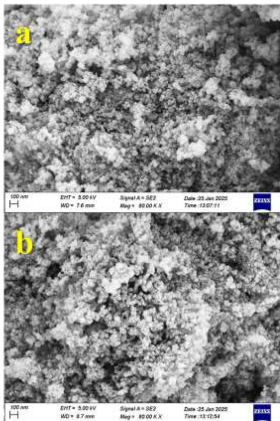
Fig. 4. FE-SEM images of a) bare n- \text{TiO}_2 -P25 and b) henna sensitized n- \text{TiO}_2 -P25.
