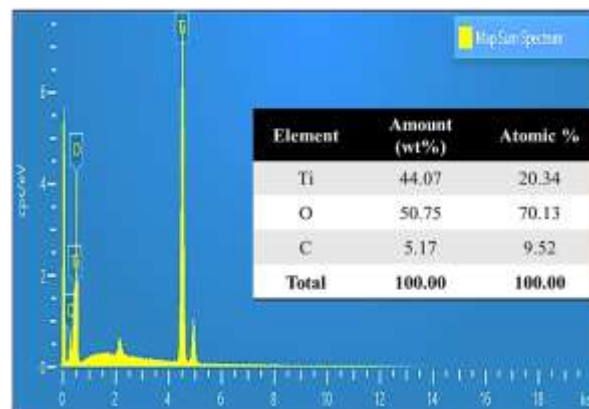
Fig. 5. EDX spectrum of henna sensitized n- \text{TiO}_2 -P25 (illustrated as element type and content analysis).
