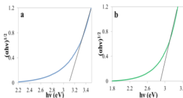
Fig. 11. Kubelka–Munk energy curve plots of a) bare n-TiO 2 -P25 and b) henna sensitized n-TiO 2 -P25.
