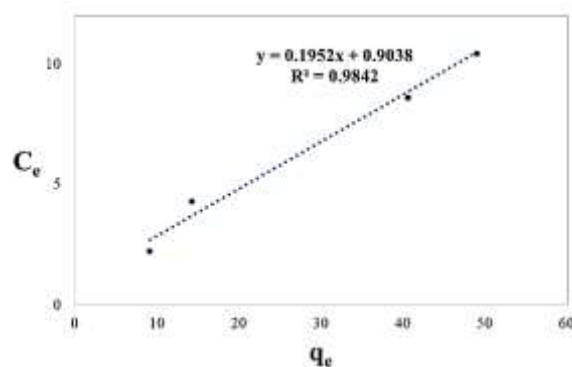
Fig. 8. Equilibrium data on the adsorption of henna dye on n-TiO 2 -P25 particles.
