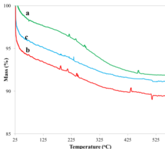
Fig. 1. TGA curves of n-TiO 2 -P25 sensitized with a) 1mg/L, b) 3mg/L, and c) 5mg/L henna.
